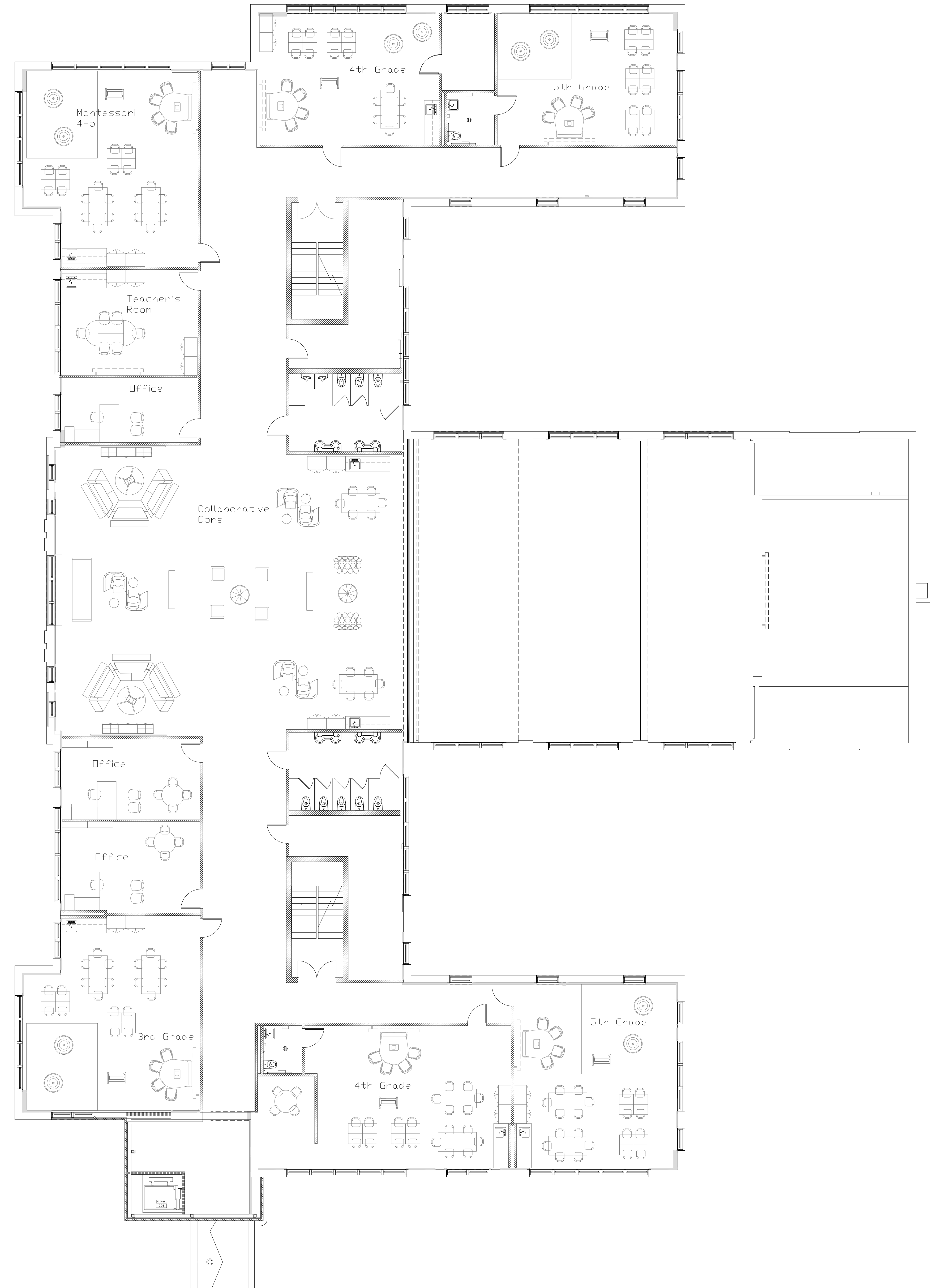
2nd Floor Building A Scale: \frac{1}{8}"=1'-0"
